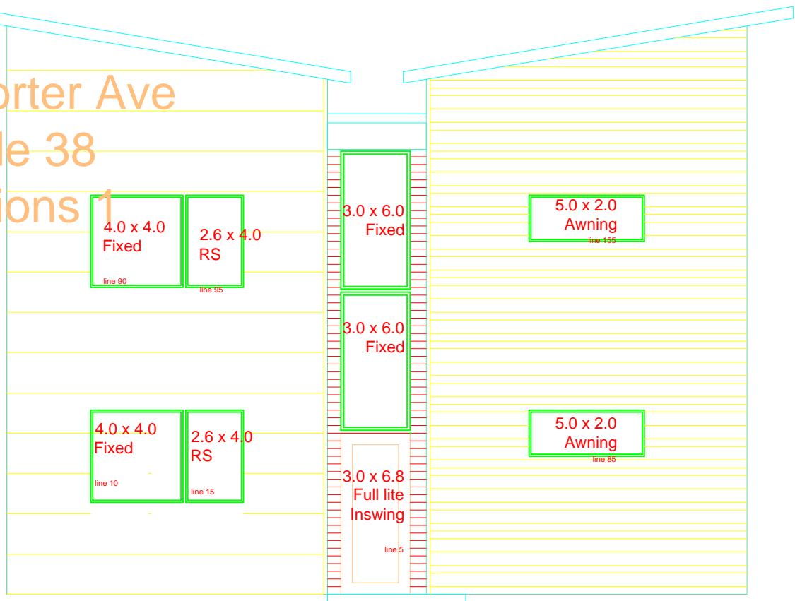
East Elevation (Front entrance)
