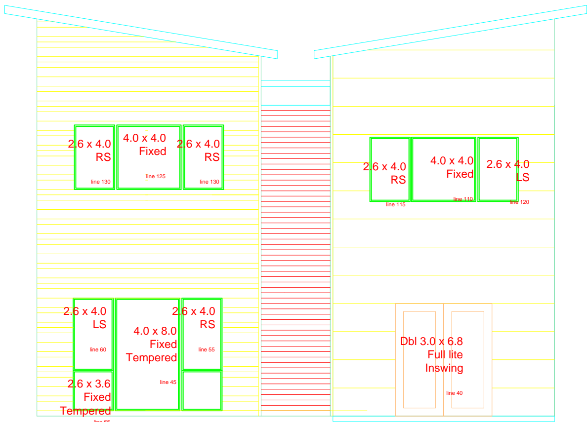
East Elevation (Front entrance)
